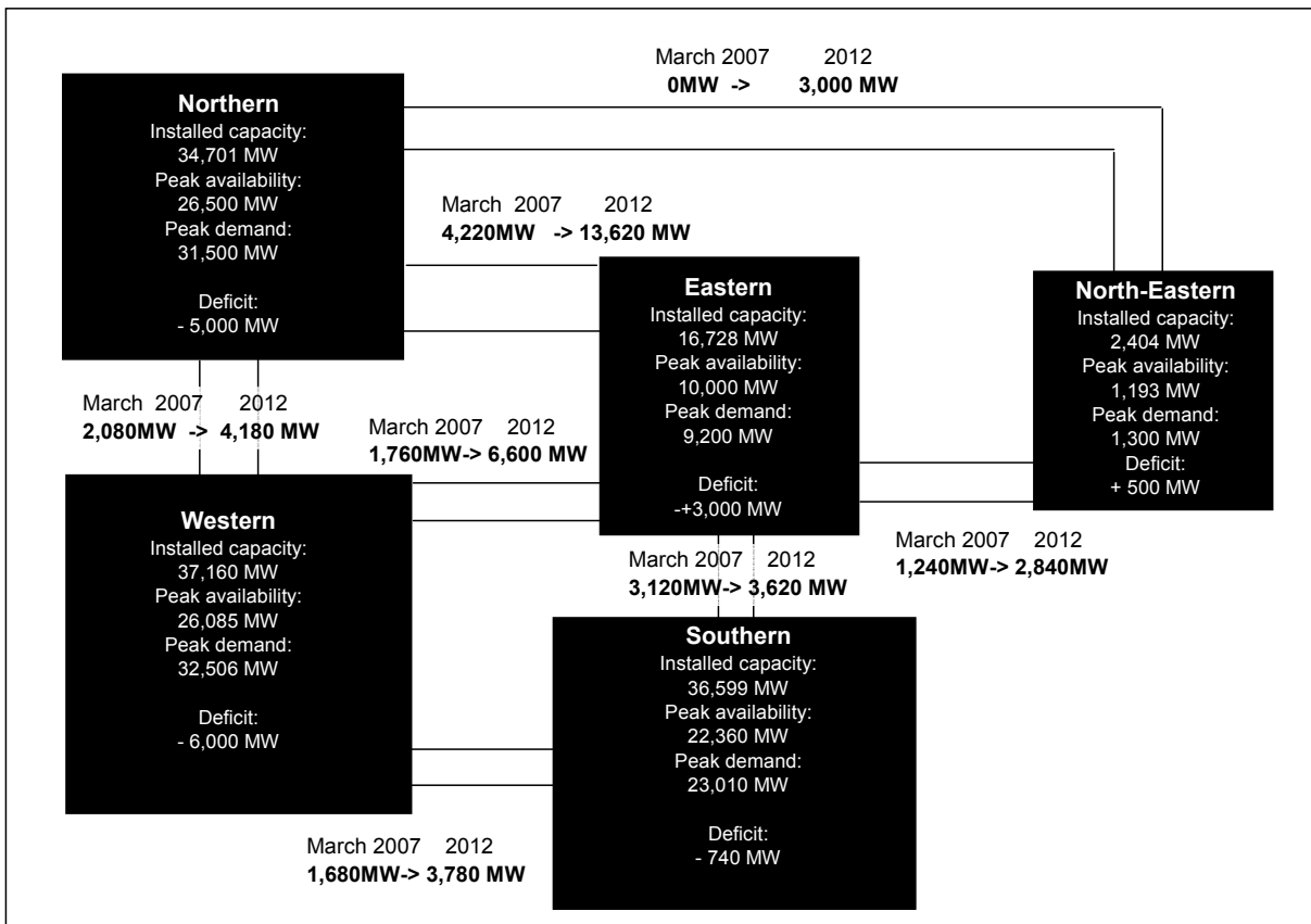
Figure 2: Proposed Interregional Transmission Capacity (MW) by 2012
