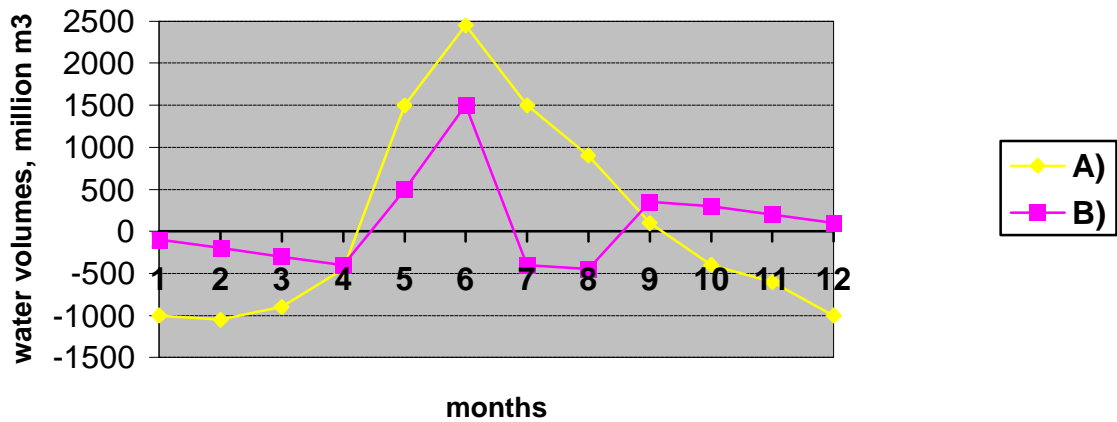
Flow Regulation to Satisfy Energy and Irrigation Demands in the Normal Year
