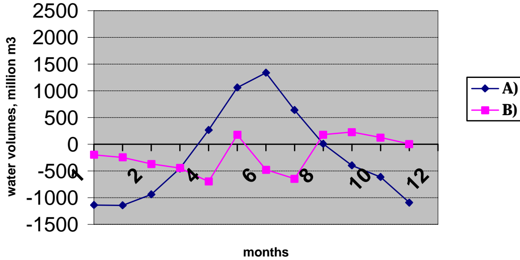
Flow Regulation to Satisfy Energy and Irrigation Demands in the Dry Year
